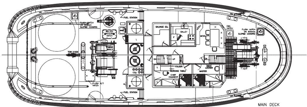
MAIN DECK
